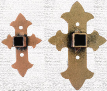
PE-10C PE-03C PE-03C4M 50x80x2mm. 75x113x2mm. 75x113x4mm. [10x10mm.] [12x12mm.] [12x12mm.]
